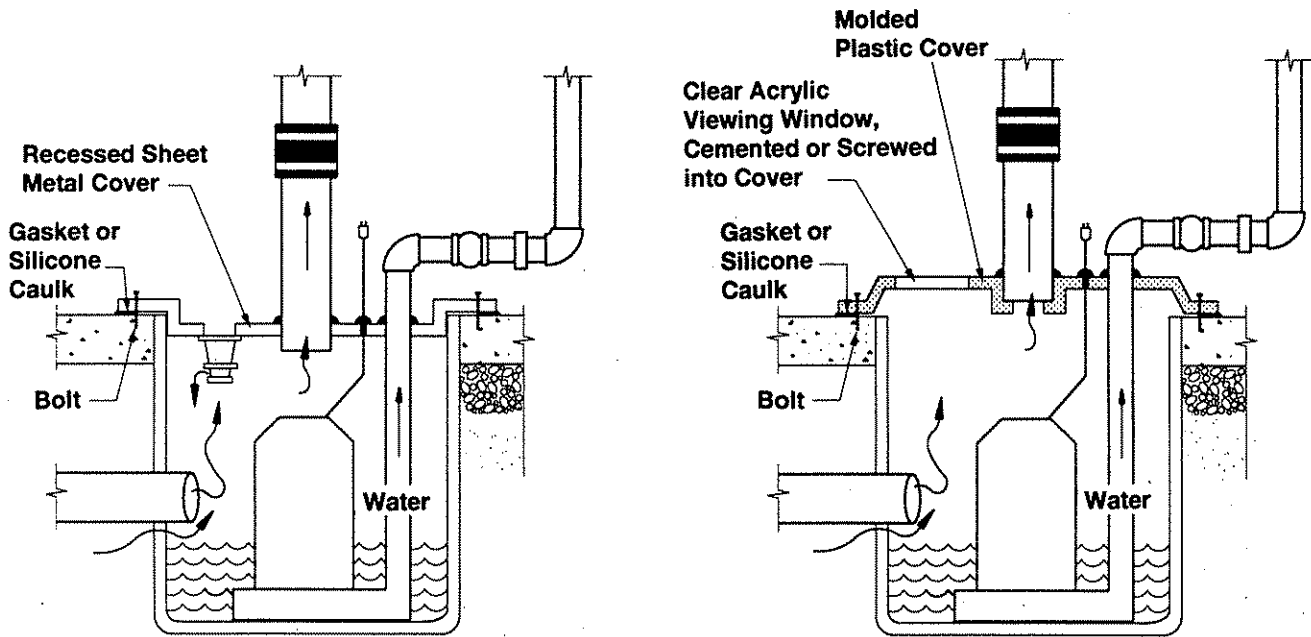
B) Recessed cover designed to be supported by top of slab.
